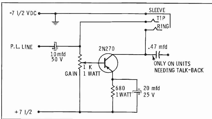
Fig. 1. Photos and circuit diagram of transistorized amplifier unit.
