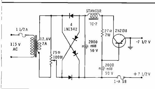
Fig. 6. Power supply serves all units.
