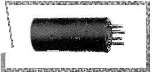
Typical Tarzian rectifiers to replace tube types 80, 82, 83, 83V, 5Z3, 0Z4, 5X4, 5Y4, 6AX5, 6X5, 866, 866A, 3B28, 6AU4, 6AX4, 6BL4, 6W4, 12AX4, 17AX4, 25W4, 6U4, and 5R4 (approximately 1/2 size)
