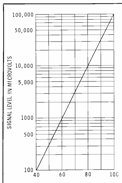
Fig. 2. New conversion scale for dbu's
