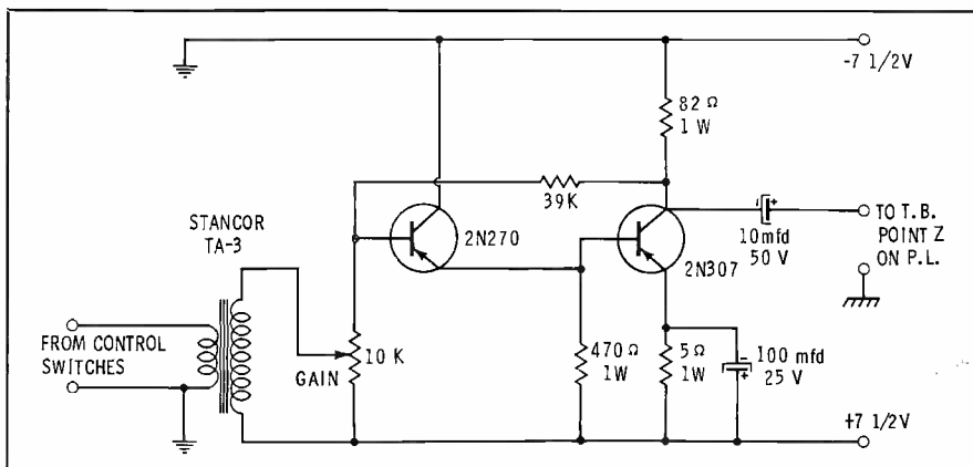
Fig. 5. Two-transistor talk-back amplifier circuit.
