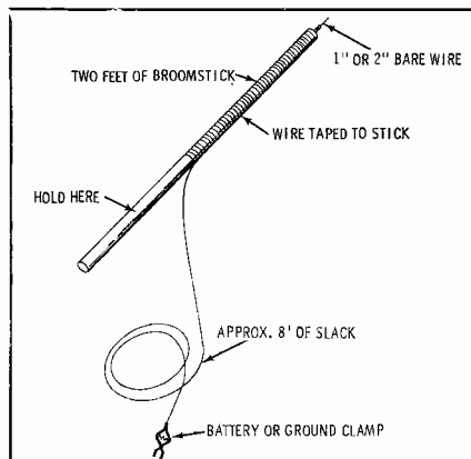
Fig. 5. Grounding stick can be made from simple materials, and may save your life.
